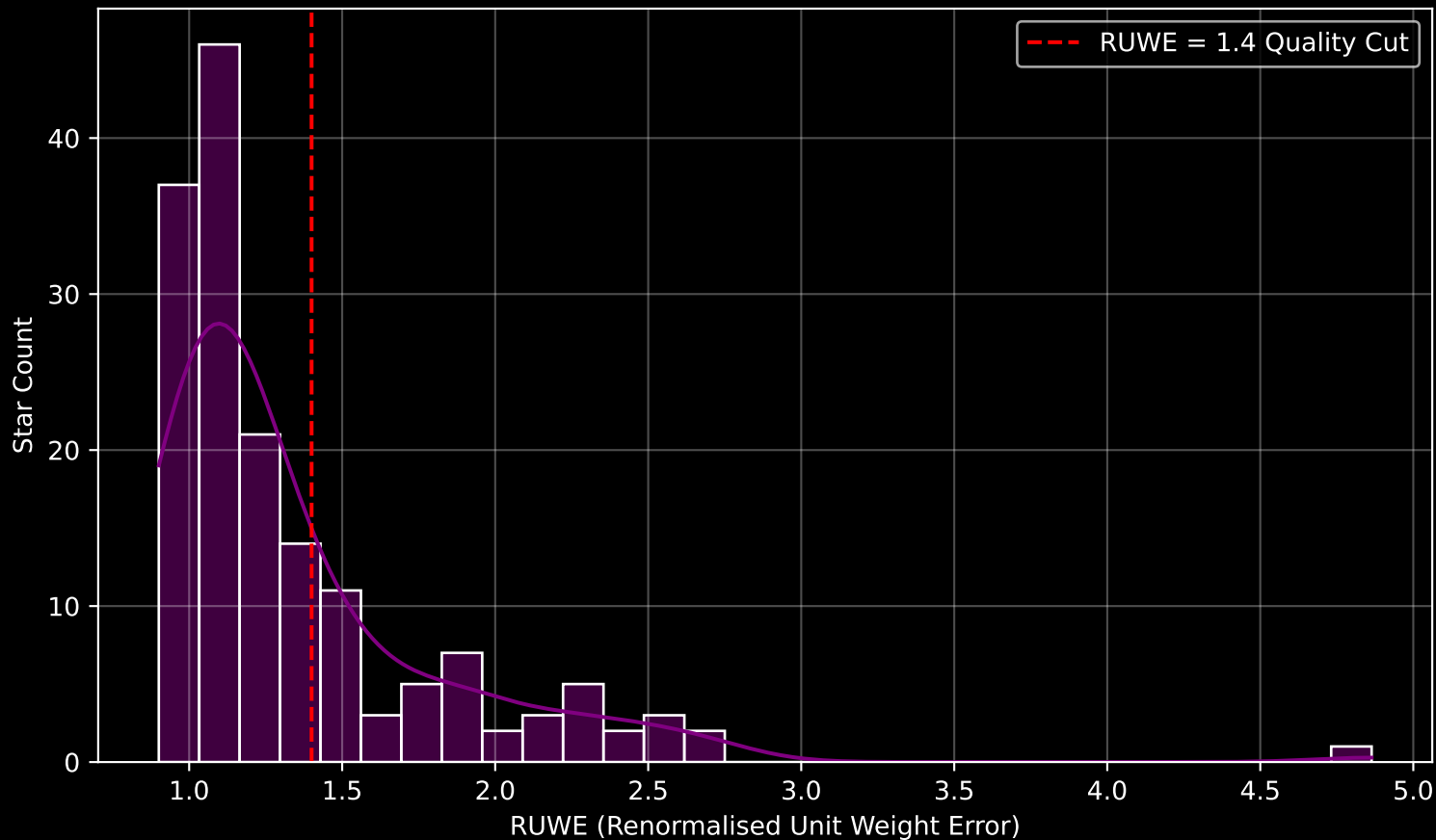
GAPOGEE DR17 Field [096+84_MGA] RUWE Distribution (n= 162)
