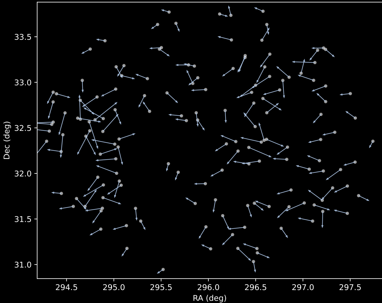
APOGEE DR17 Cluster 1 Proper Motion Vectors (n=151)
