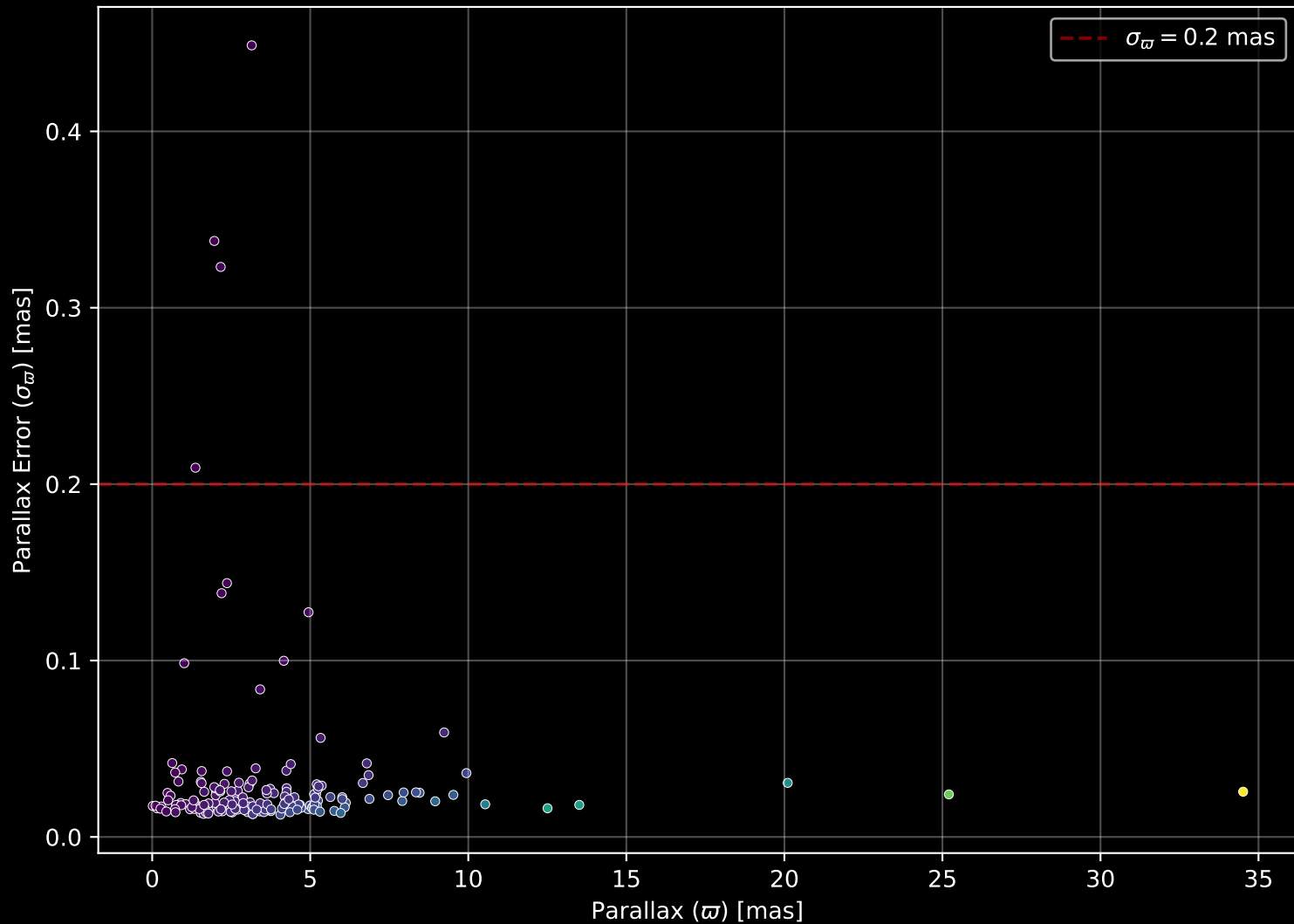
APOGEE DR17 Field: [096+84_MGA] Parallax Quality (n= 171)
