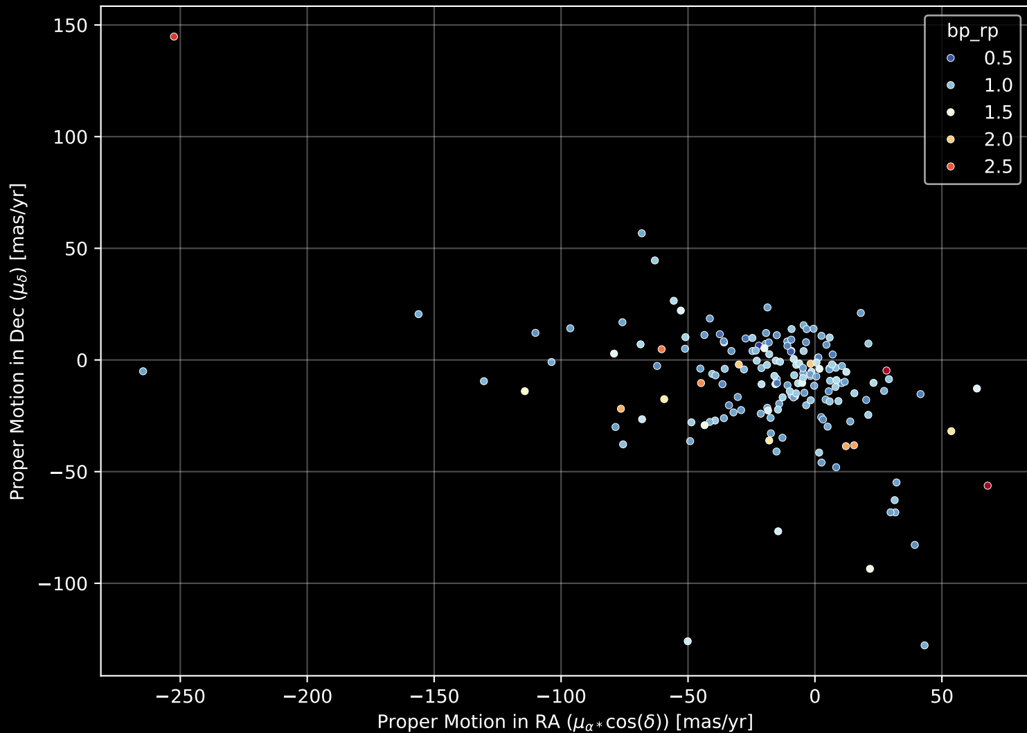
APOGEE DR17 Field: [096+84_MGA] Proper Motion Diagram (n= 171)
