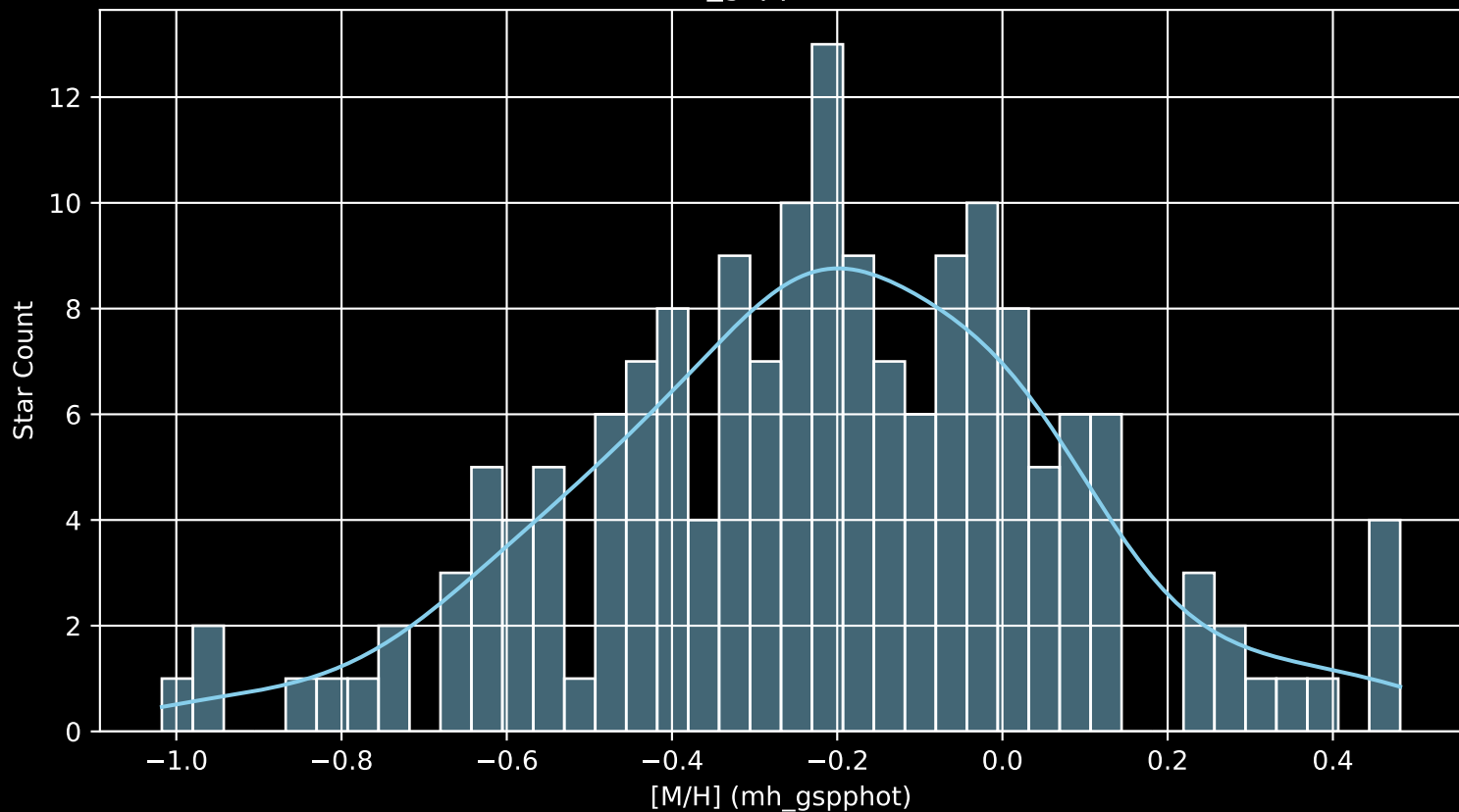
APOGEE DR17 Field: [096+84_MGA [M/H] (mh_gspphot) (n= 168)
