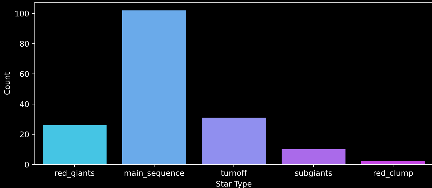
APOGEE DR17 Field: [096+84_MGA] Count plot of Star Type
