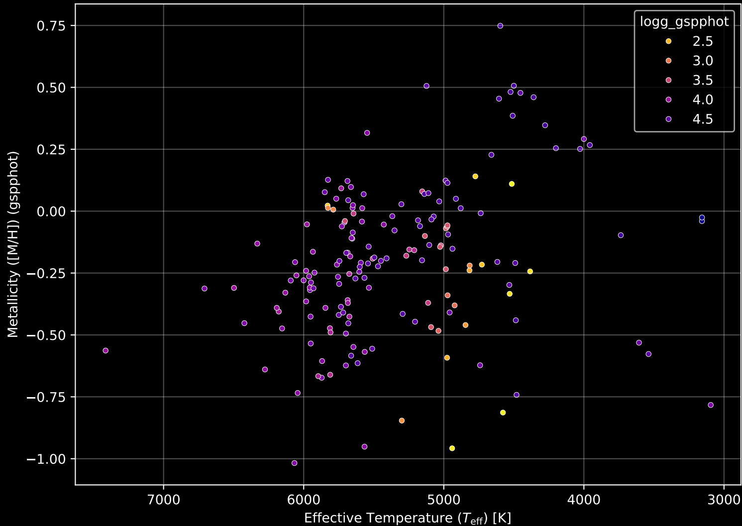
APOGEE DR17 Field: [096+84_MGA] Stellar Population Parameters (n= 171)
